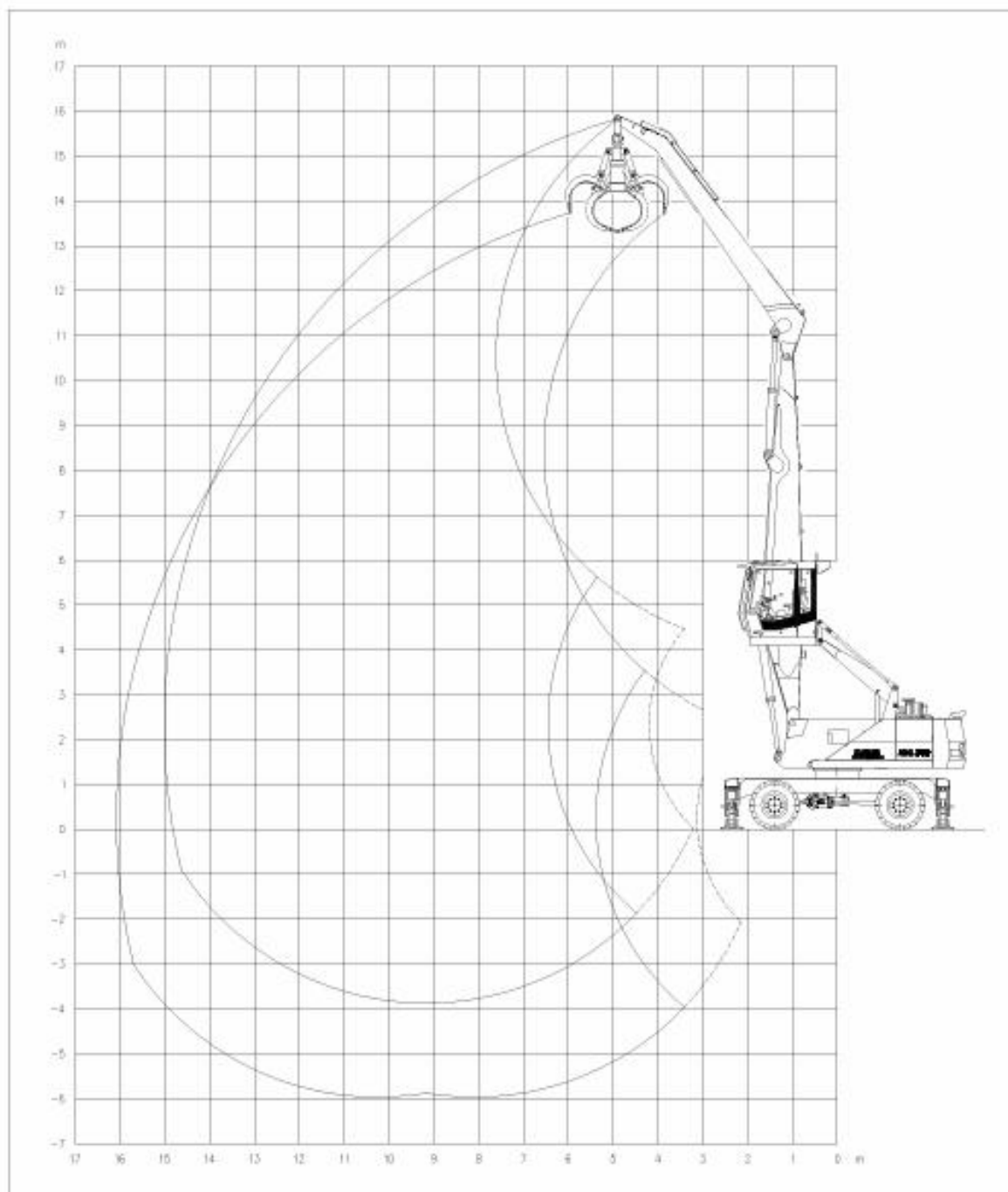
Fig. 9 Working range diagram (15 m loading equipment)
